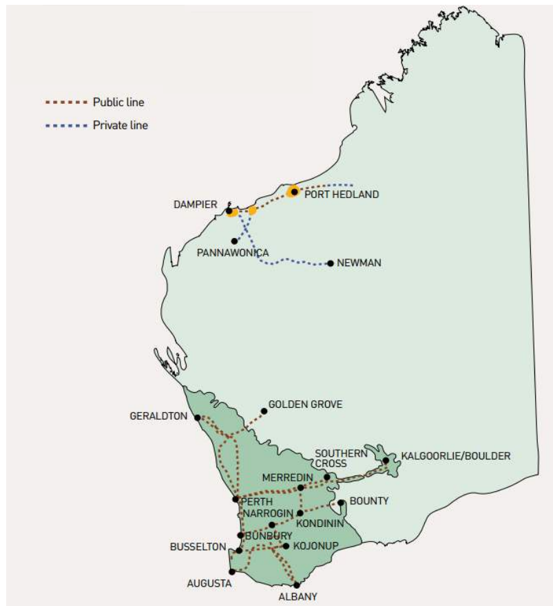
Electricity infrastructure map, Western Australia
